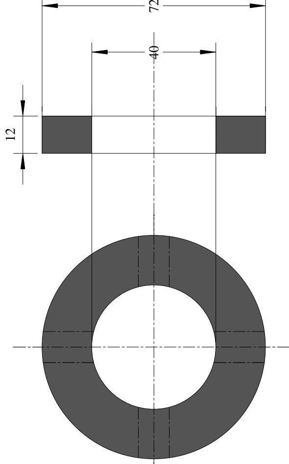
Steel collar for the oneway bearing
